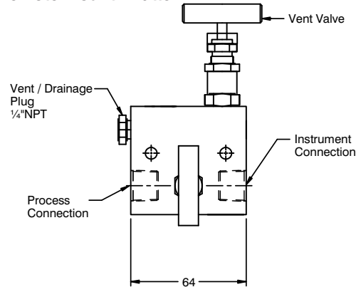
Remote mount - Pattern 1
