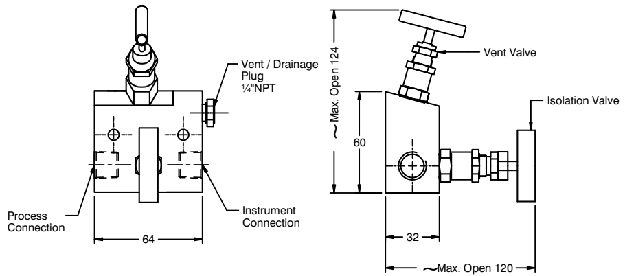
Remote mount - Pattern 3
