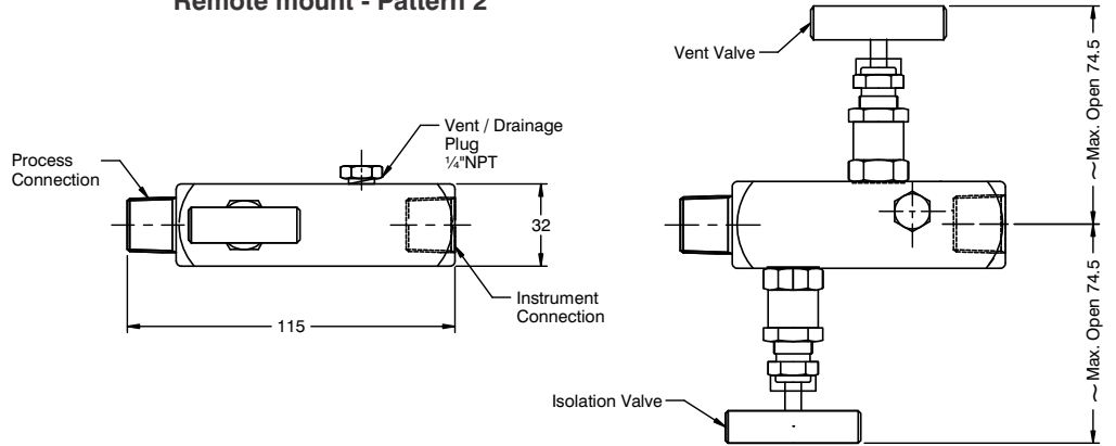
Remote mount - Pattern 2
