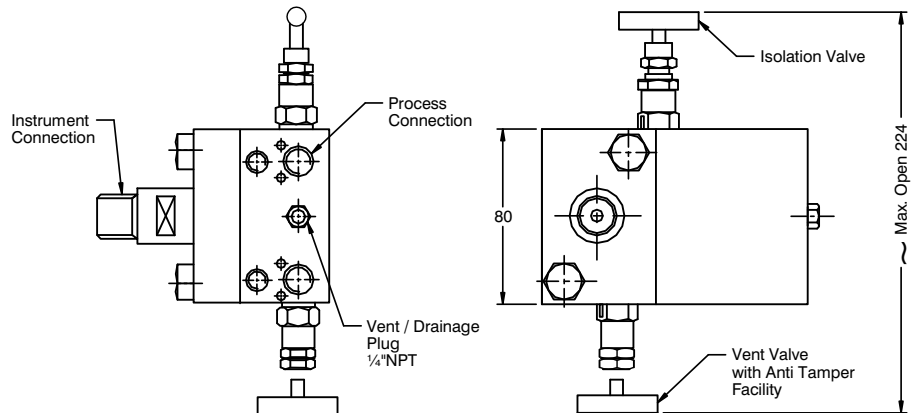
Direct mount - Pattern 4
