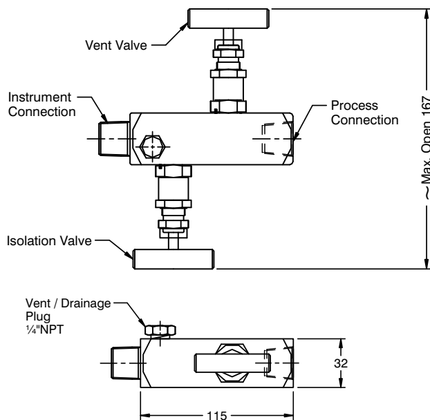
Remote mount - Pattern 4
